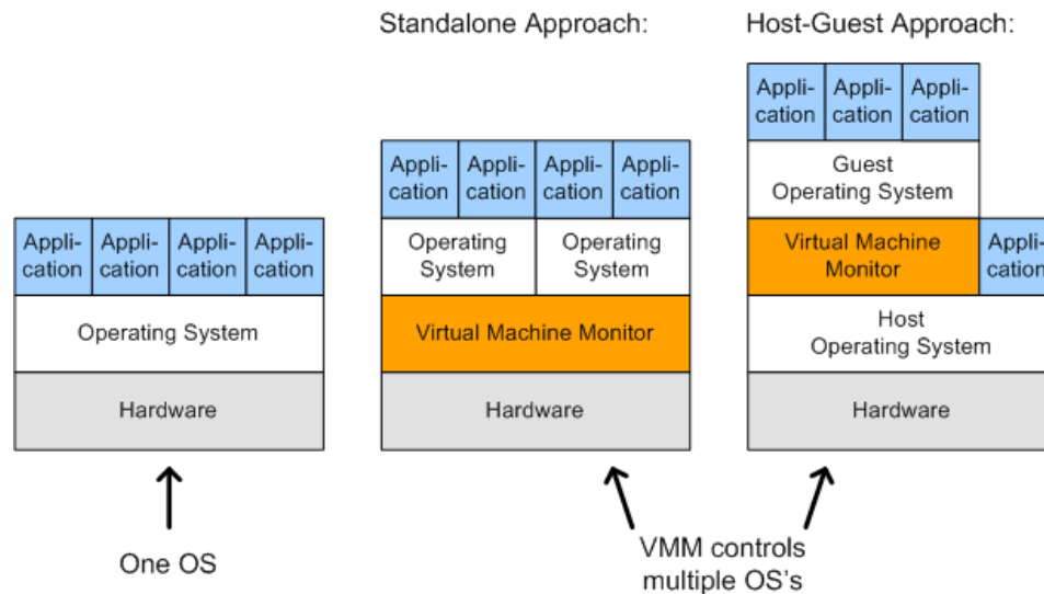
Figure 3 Virtualization Styles
