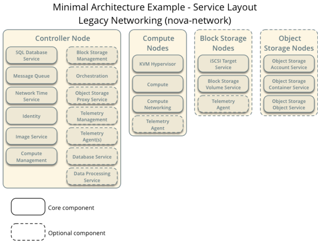
Figure 1.7. Minimal architecture example with legacy networking (nova-network)—Service layout
