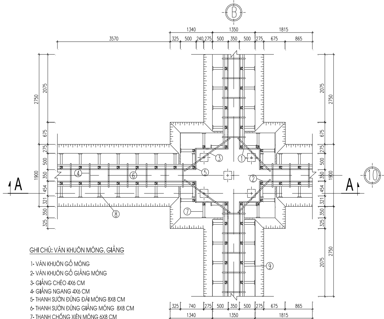
v, n khu«n ®µi mǎng m1-b (t l :1/100)
