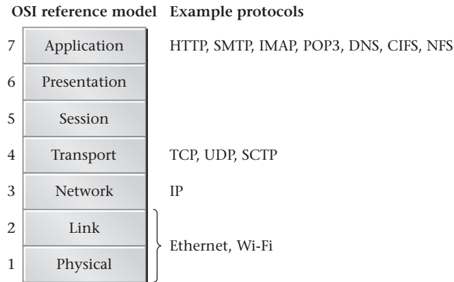
Figure 9.3: This diagram of the seven protocol layers in the OSI reference model provides examples for the layers I discuss.
