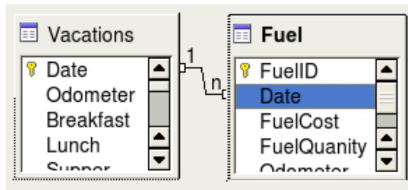
Figure 9: Designation for a 1:n relationship
